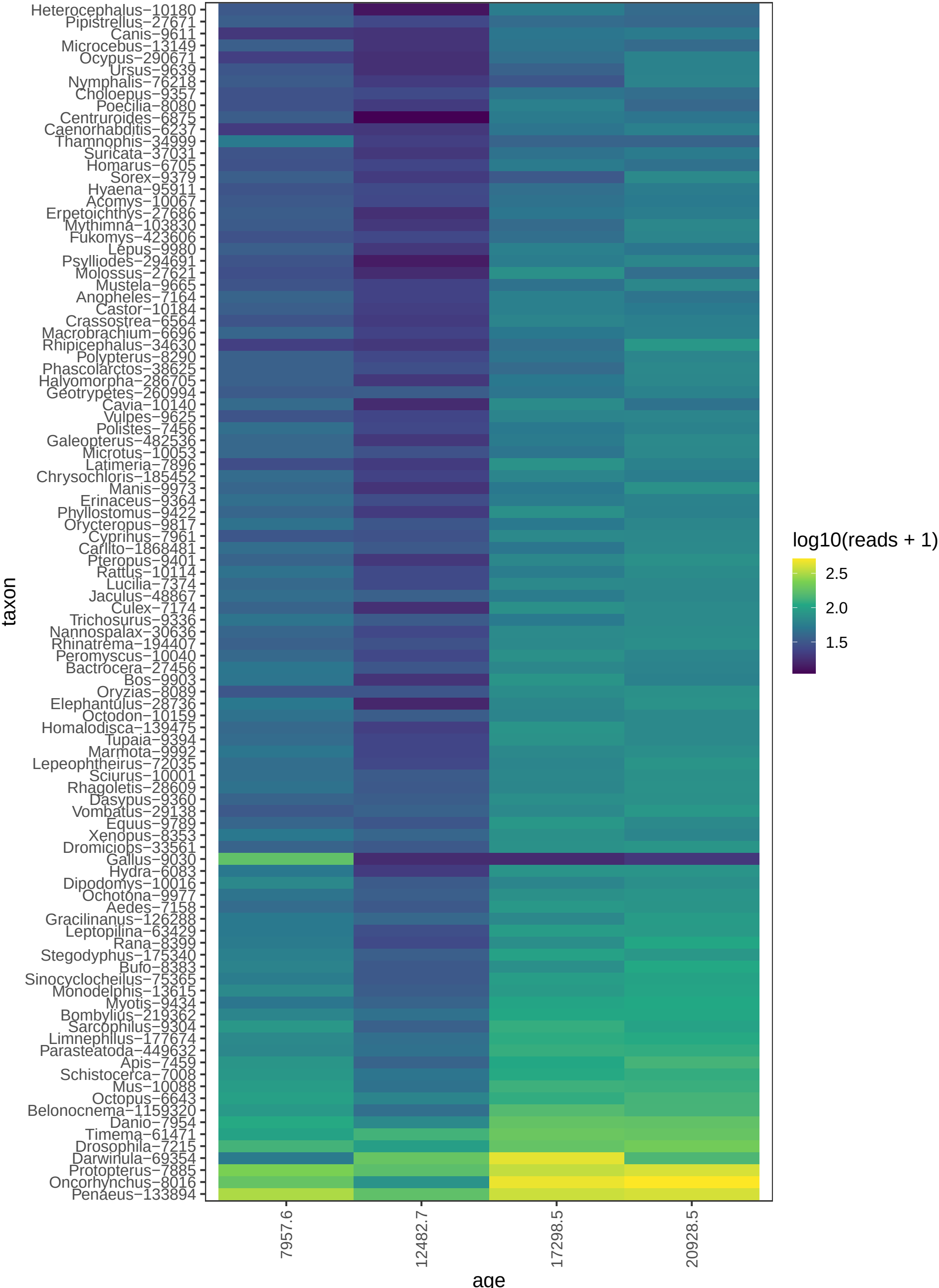
stable – Top 100 Genera in Hashilan marsh ( animal )
